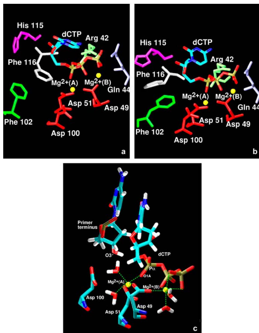
FIGURE 8 Active site of the ternary complex (pol X-DNA-dCTP) ( a ) before and ( b ) after 10.5 ns of molecular dynamics (simulation 7). ( c ) Coordination spheres for the catalytic ( A ) and nucleotide binding ( B ) magnesium ions at the end of the dynamics trajectory.
