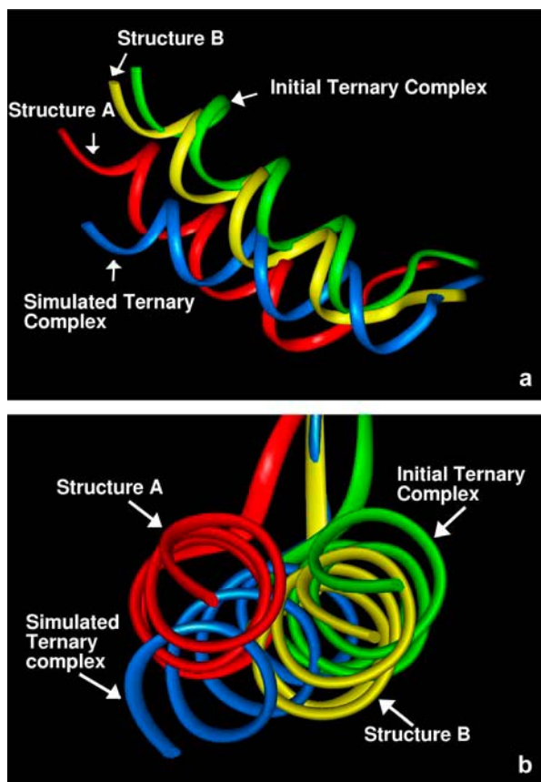
FIGURE 7 Comparison of the simulated ternary structure at isotonic conditions (blue, simulation 7) with the free pol X structures: free pol X structure A (initially closed) is shown in red, free pol X structure B is shown in yellow, and the equilibrated initial ternary model is shown in green. The structures are superimposed on the C \alpha atoms of the palm subdomain (residues 1–105). Only helix E and adjacent residues (117–132) are shown in the pictures. (a) Lateral view; (b) front view.
