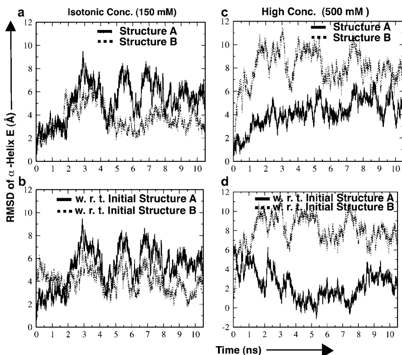
FIGURE 3 RMSD plots for helix E of the free pol X structures obtained by superimposing the palm (residues 1–105) for simulations performed at physiological, 150 mM ( a and b ) (simulations 1 and 2), and high salt concentration, 500 mM ( c and d ) (simulations 3 and 4). ( a ) Time evolution plots of the RMSD values for both structure A (initially closed) and structure B (initially open) with respect to initial conformation at physiological conditions. ( b ) RMSD values obtained by superimposing the palm of structure A in the trajectory with initial structure A and initial structure B. This plot clearly shows that final structure A (at the 10 ns) superimposes better with structure B (average RMSD for the final 2 ns \sim 3.5 Å) than with the initial structure A (average RMSD for the final 2 ns \sim 5.5 Å). ( c ) Time evolution plots of the RMSD values for both structure A (initially closed) and structure B (initially open) with respect to initial conformation at high salt. ( d ) RMSD of structure B plotted with respect to its starting conformation and with respect to structure A. RMSD with respect to structure A is corrected for translational motion following earlier works (see Arora and Schlick (61)) and shows that the final structure B superimposes better with structure A than with initial structure B.
