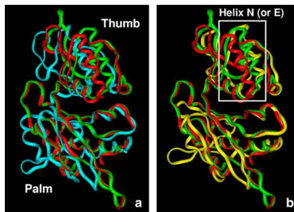
FIGURE 1 Comparison of the structures of human pol \beta with the NMR-determined structures of pol X. For pol \beta , only residues 145–335 (corresponding to the palm and thumb domain) are shown. In both figures, the open conformation of pol \beta (1BPX) is represented in green and the closed conformation (1BPY) is in red. In panel a , pol \beta structures are compared with free pol X structure A (initially closed) (41), and in panel b , pol \beta structures are superimposed with pol X structure B (initially open) (42). The inset identifies the region of proteins where most of the differences lie (helix N for pol \beta , and helix E for pol X. Residues of the catalytic triad and adjacent ones are used in the superimposition (residues 49–51 and 99–101 for pol X; residues 190–192 and 255–257 for pol \beta ).
